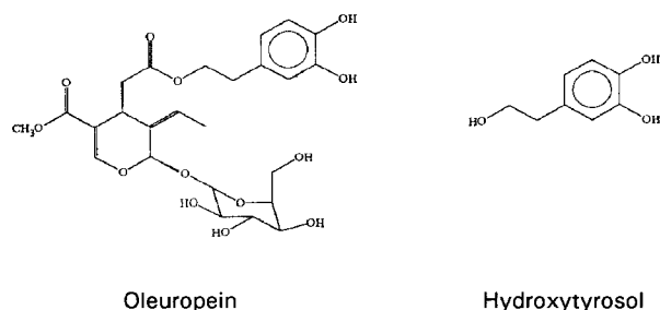
Figure 1 The structural formulae of oleuropein and hydroxytyrosol.
