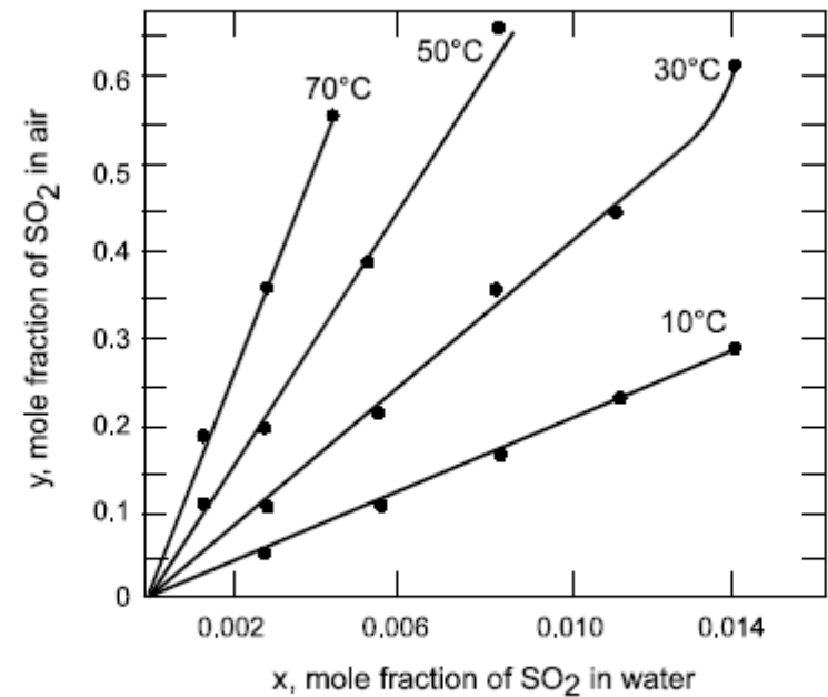
Figure 11-1. Equilibrium lines for SO 2 - H 2 O systems at various temperatures
