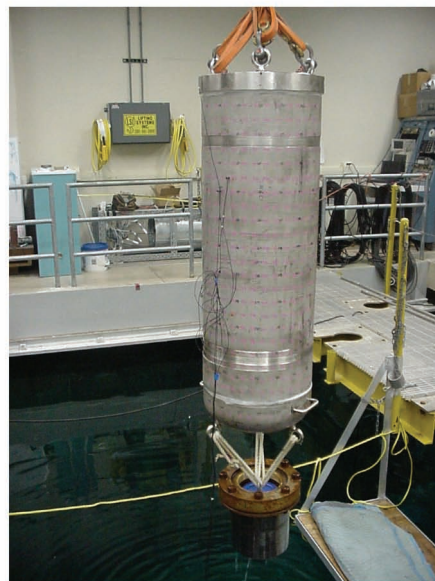
Fig. 13. Impact hammer measurements on cylindrical shell structure submerged in ARL/Penn State Reverberant Water Tank. Top—shell submerged in tank with diver; bottom, shell suspended over tank.
