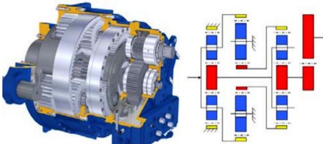
Fig. 4 Differential gearbox, Bosch Rexroth, working principle
