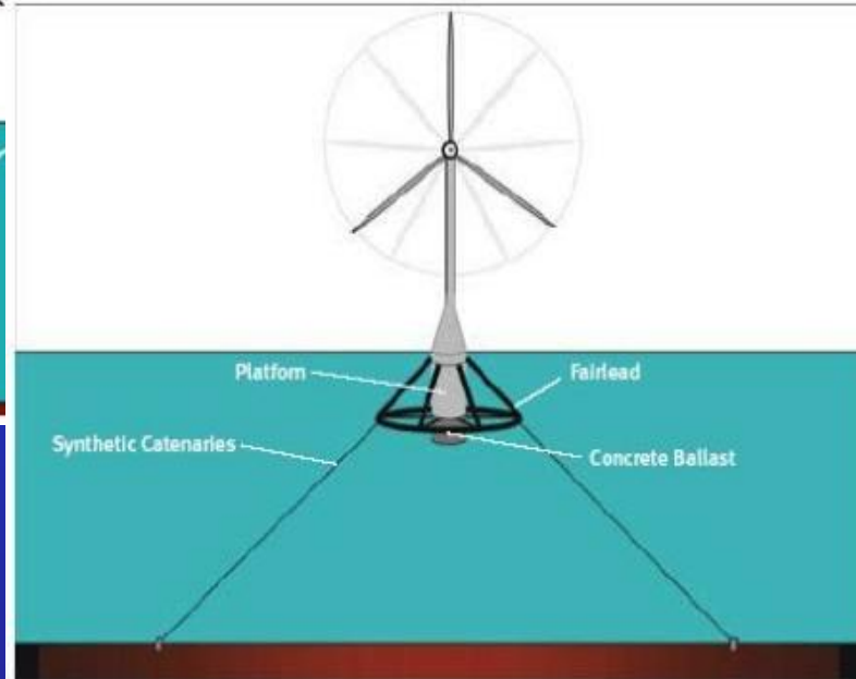
HYBRID TLP-SPAR FLOATER WITH TAUGHT CATENARIES
