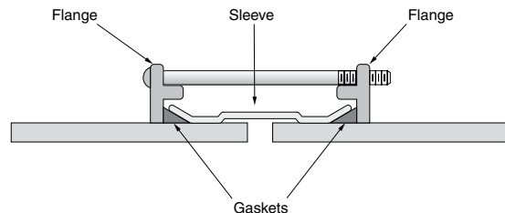
Figure 12-11 Mechanical Steel Coupling
