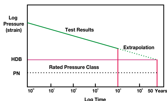
Figure 3-2 Test Results evaluation -ASTM Test procedure B
