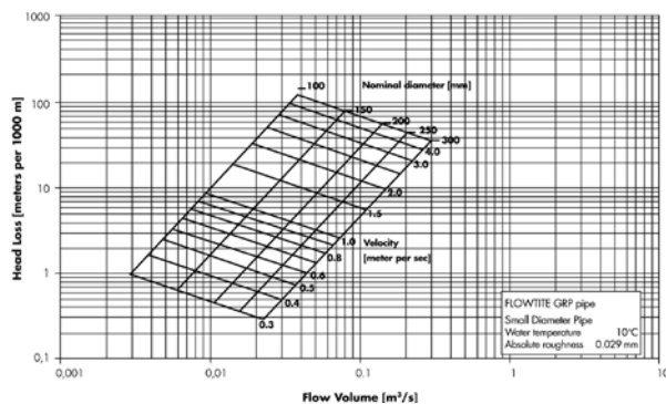
Figure 4-1 Head Loss – Small Diameters
